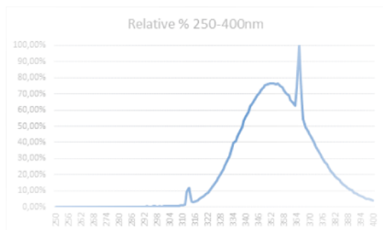
PL-L 36W09 UVA Spectral distributiin graph
